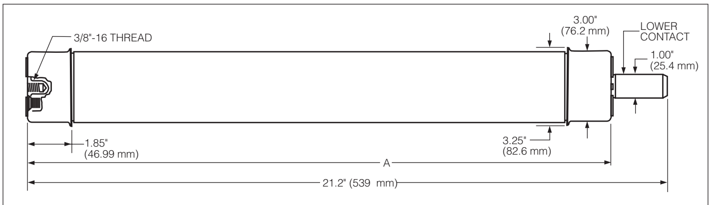
Figure 9. Dimensional information for E-rated 15.5 kV (65E-100E) version ELSG fuses.
