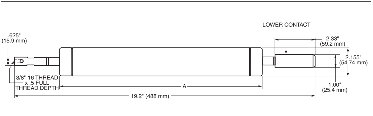
Figure 4. Dimensional information for single 2" diameter 8.3 kV and 15 kV E-rated and MSLE version ELSG fuses.
