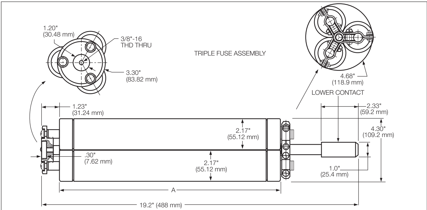
Figure 7. Dimensional information for E-rated 15.5 kV (150E) version ELSG fuses.
