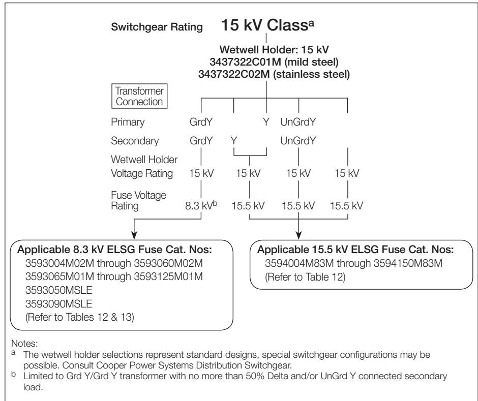
Figure 13. Fuse Selection Guide for 15 kV Class Switchgear.
