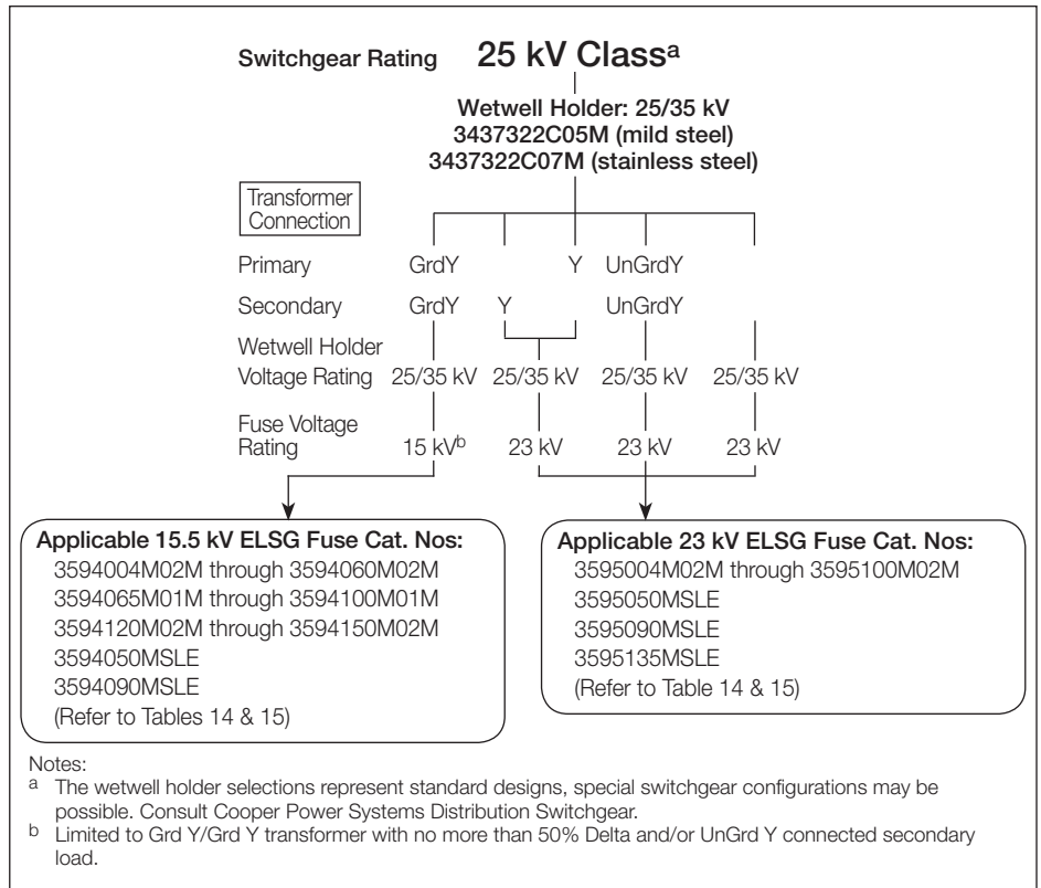
Figure 14. Fuse Selection Guide for 25 kV Class Switchgear.
