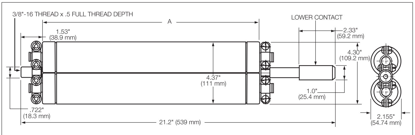
Figure 10. Dimensional information for E-rated 15.5 kV (120E) and 23 kV (50E, 65E) and 15.5 kV and 23 kV (90A) MSLE version ELSG fuses.
