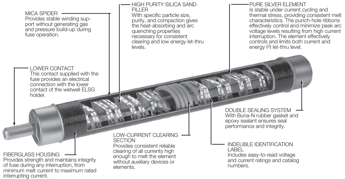
Figure 2. Cutaway illustration of the ELSG fuse.
