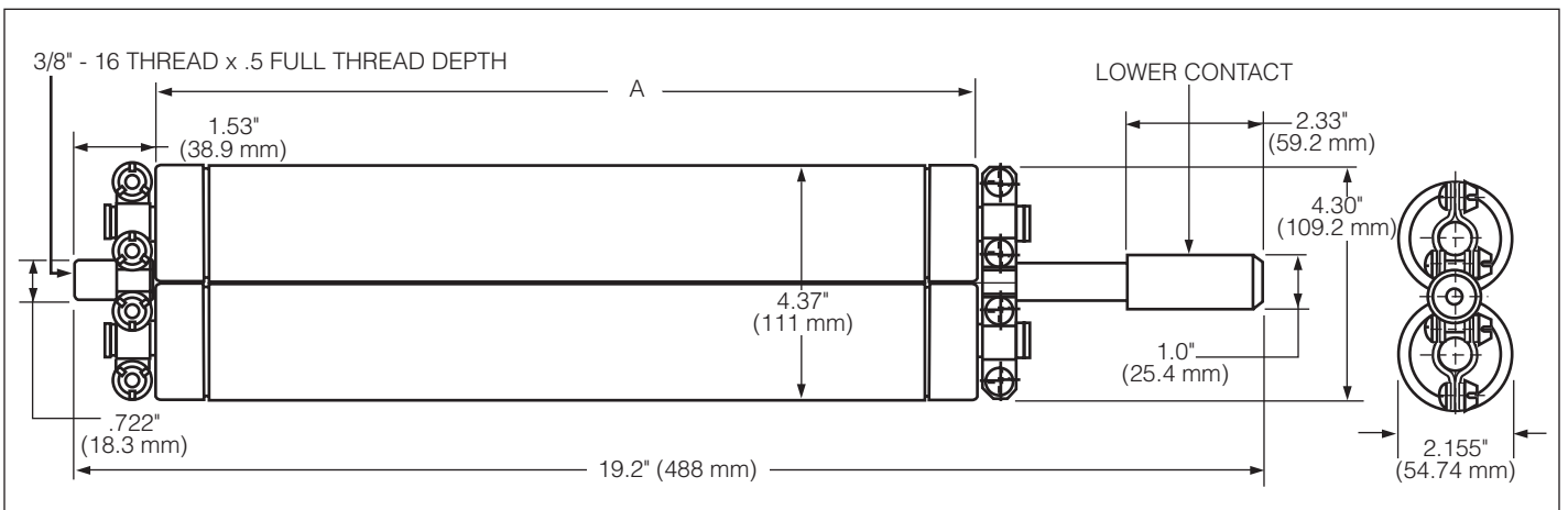
Figure 6. Dimensional information for E-rated 15.5 kV (65E-120E) and 15.5 kV (90 A) MSLE version ELSG fuses.
