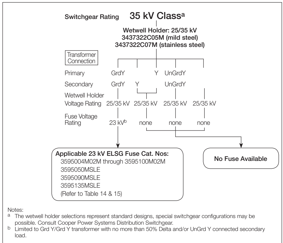
Figure 15. Fuse Selection Guide for 35 kV Class Switchgear.
