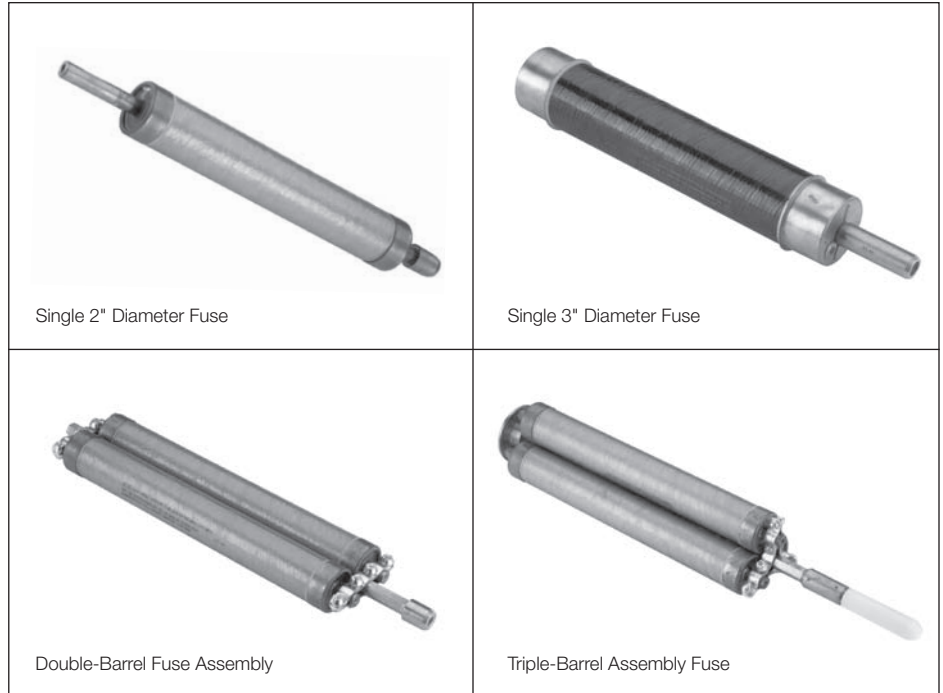
Figure 1. ELSG Current-Limiting fuses.
