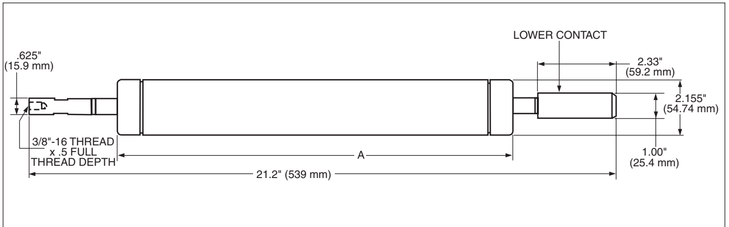
Figure 8. Dimensional information for single 2" diameter 15 kV and 23 kV E-rated and MSLE version ELSG fuses.
