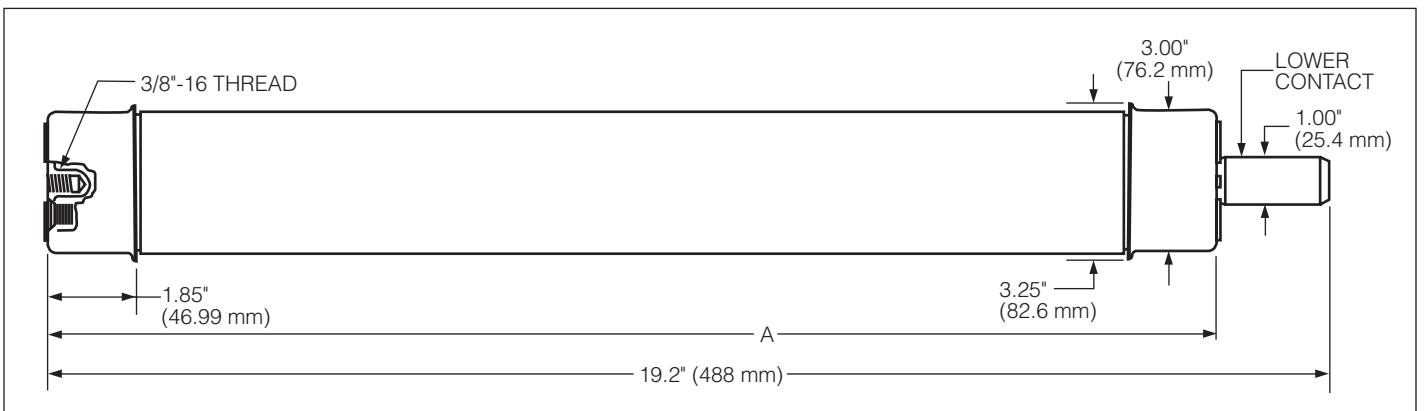
Figure 5. Dimensional information for E-rated 8.3 kV (65E-125E) version ELSG fuses.
