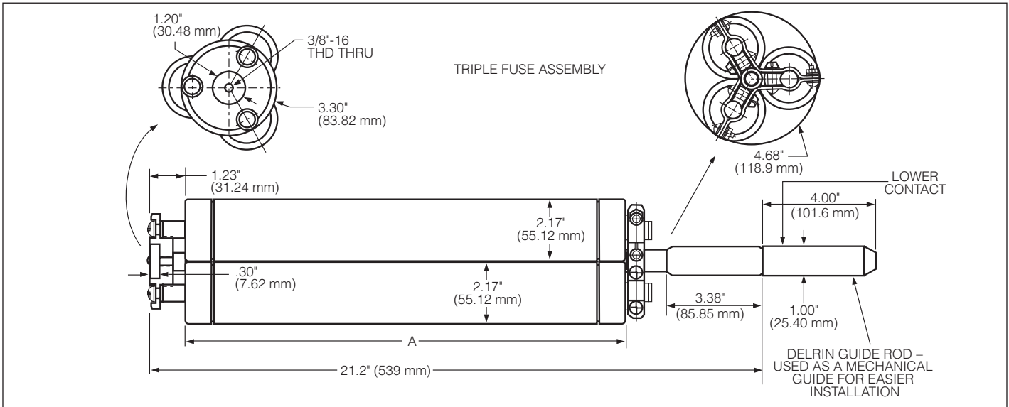
Figure 12. Dimensional information E-rated 23 kV (80E, 100E) and MSLE 23 kV (135A) version ELSG fuses.
