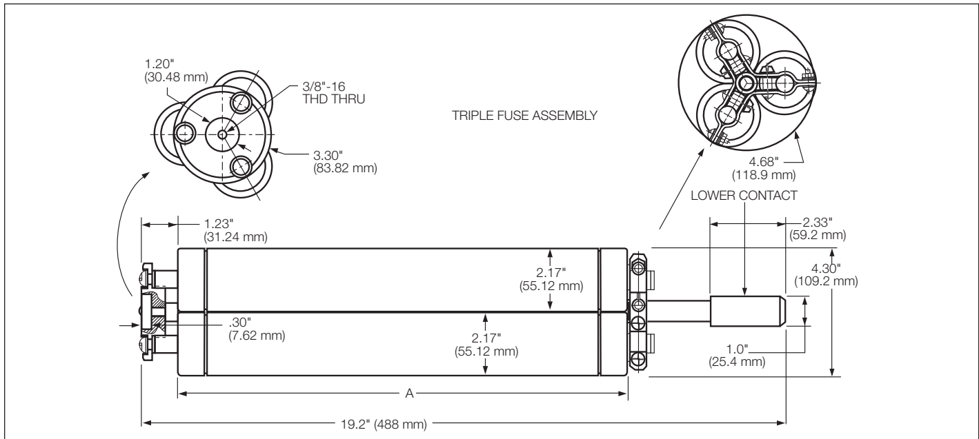
Figure 11. Dimensional information for E-rated 15.5 kV (150E) version ELSG fuses.
