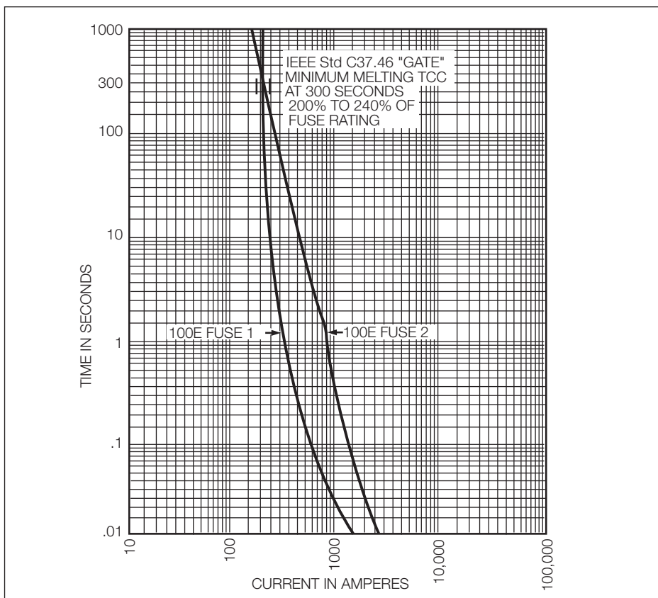
Figure 3. 100E rated current-limiting fuse “gate” per IEEE.
