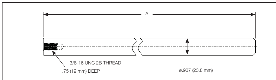
Figure 16. Dimensional Information for Shorting Bar.
